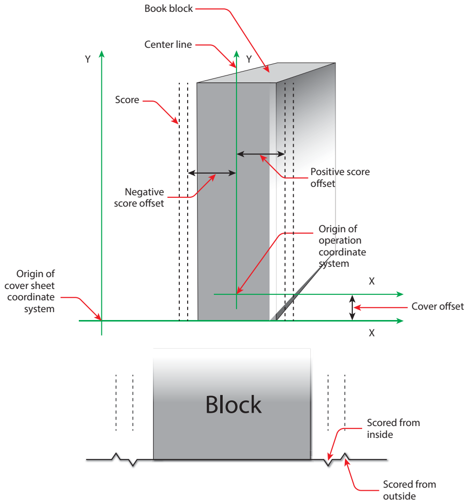
Figure 6-13: Parameters and coordinate system for cover application
