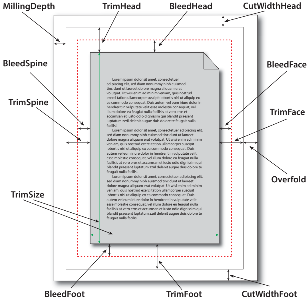
Figure 6-3: Definition of margins in SignatureCell
