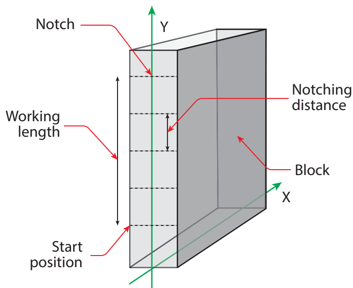
Figure 6-38: Parameters and coordinate systems for the SpinePreparation process
