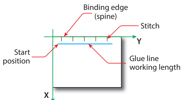
Figure 6-45: Parameters and coordinate system used for thread sewing
