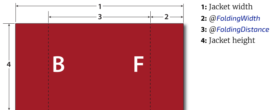
Figure 6-25: Parameters and coordinate system for jacking
