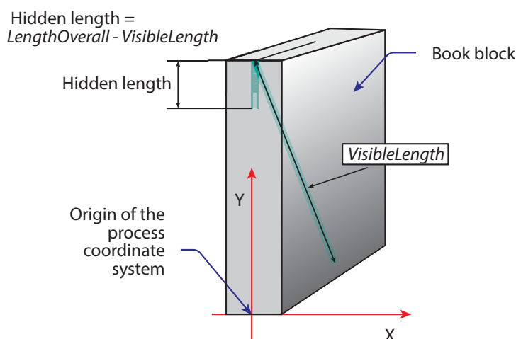
Figure 8-2: RegisterRibbon lengths and coordinate system for BlockPreparation
