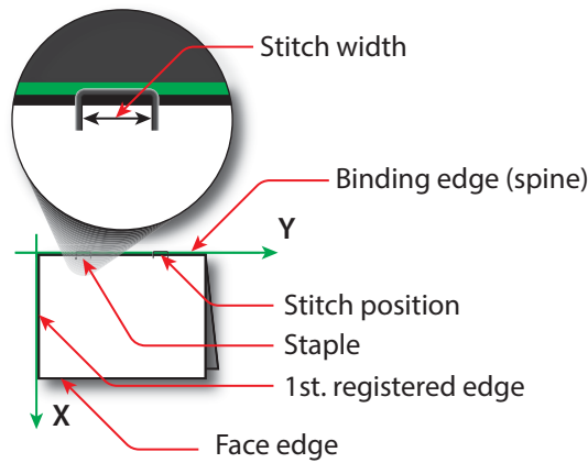
Figure 6-40: Parameters and coordinate system used for saddle stitching
