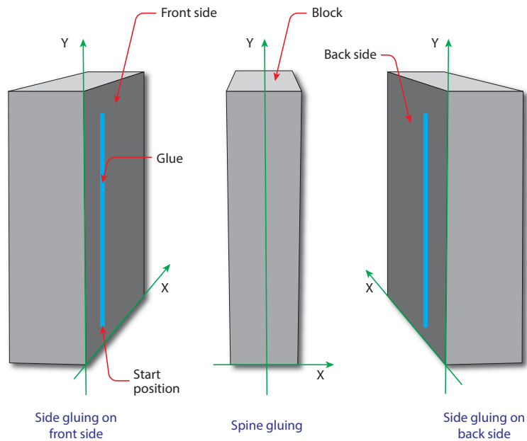
Figure 6-14: Parameters and coordinate system for glue application
