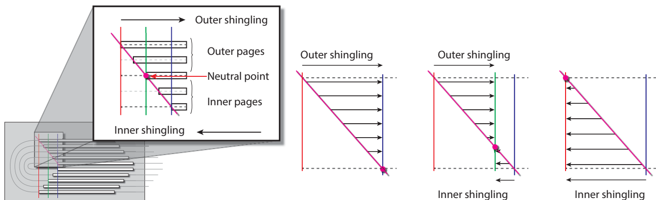
Figure 6-28: Shingling for stripping – details
