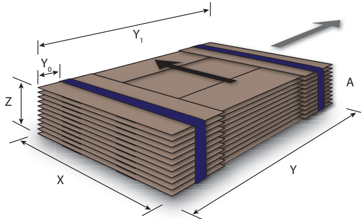
Figure 6-44: Strapped bundle with sub-bundles
