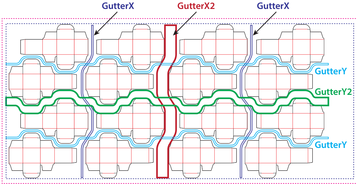
Figure 6-22: RepeatDesc using Secondary Gutters
