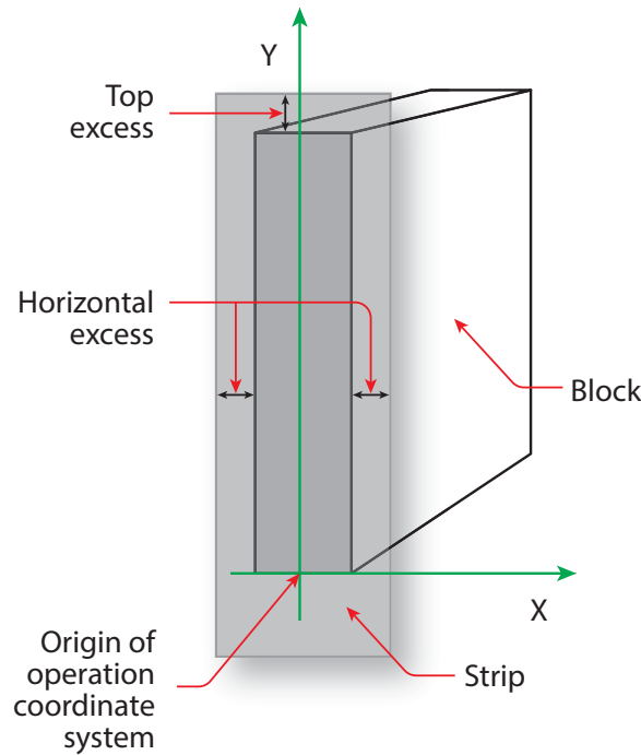
Figure 6-39: Parameters and coordinate system for the SpineTaping process
