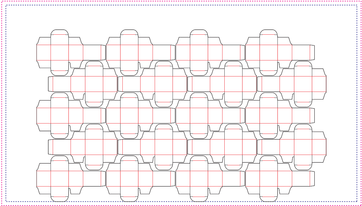
Figure 6-18: RepeatDesc/@LayoutStyle = "Reverse2ndRow"
