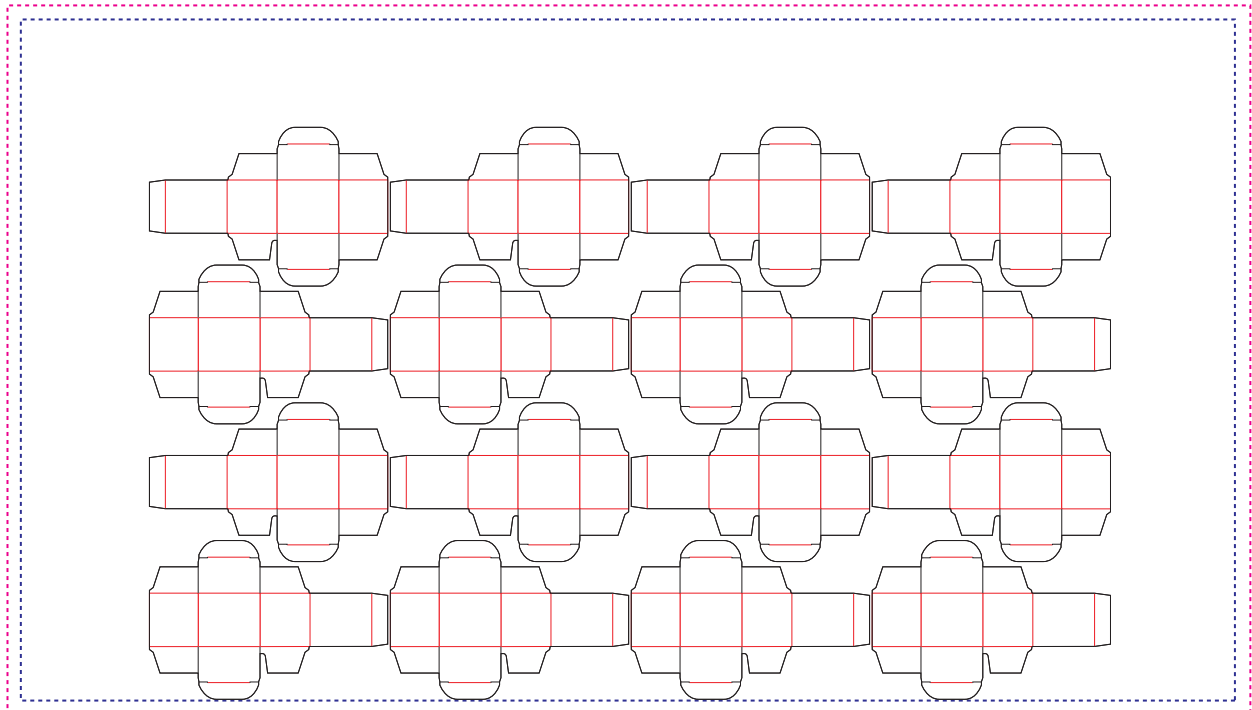
Figure 6-19: RepeatDesc/@LayoutStyle = "Reverse2ndRowAligned"
