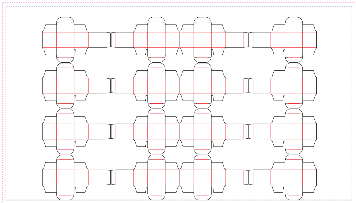
Figure 6-21: RepeatDesc/@LayoutStyle = "Reverse2ndColumnAligned"
