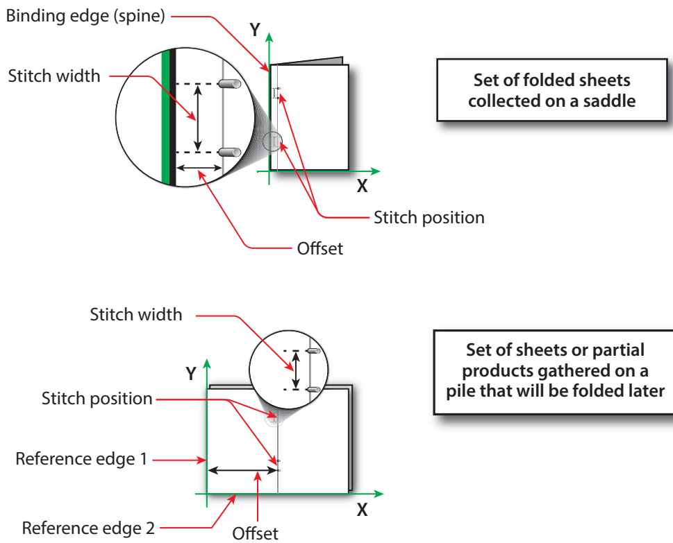
Figure 6-41: Parameters and coordinate system used for stitching
