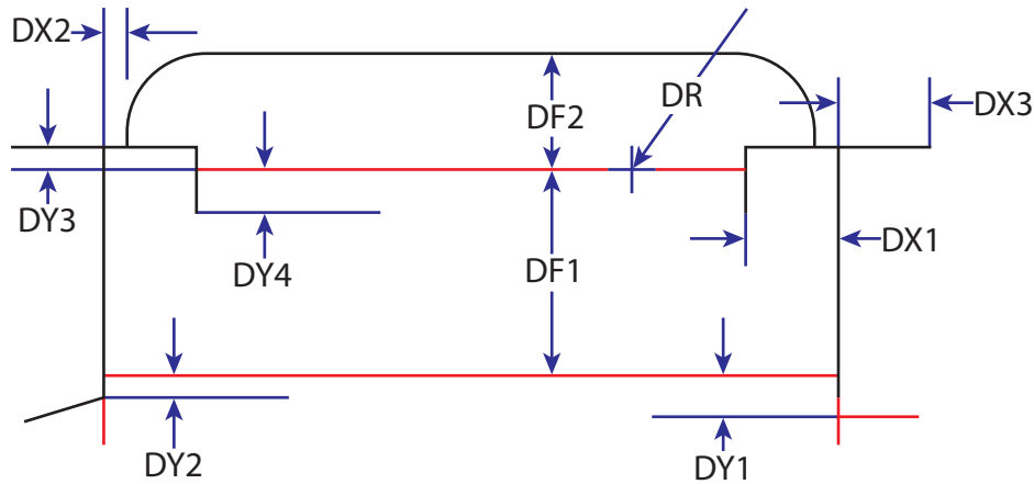
Figure 8-45: ShapeTemplate example 3
