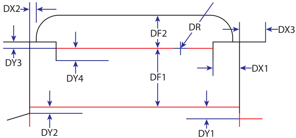
Figure 8-44: ShapeTemplate example 3
