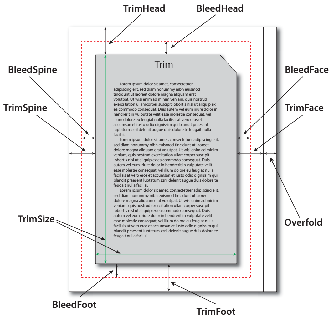
Figure 8-55: Definition of margins in StripCellParams a
