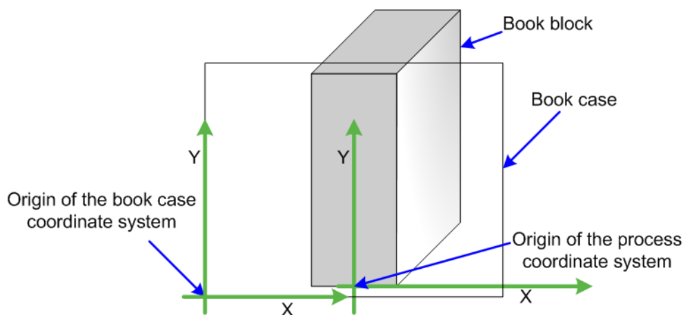
Figure 8-11: Parameters and coordinate system for CasingIn
