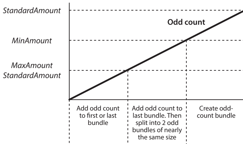
Figure 6-14: Odd count handling for a bundle
