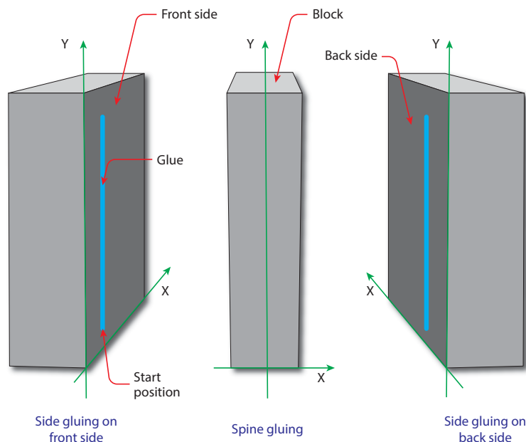
Figure 8-30: Parameters and coordinate system for GlueApplication
