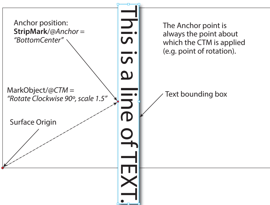
Figure 9-3: Anchor with 1.5 scaling and rotation of 90° clockwise
