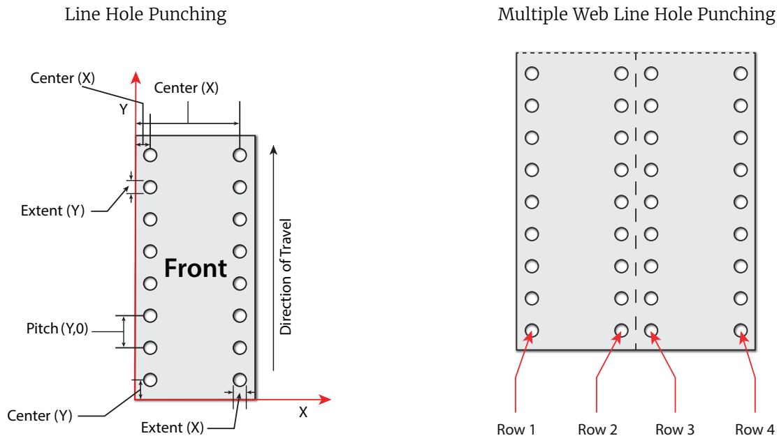
Figure 6-10: Hole parameters
