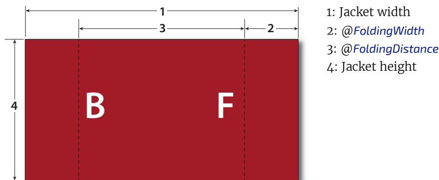
Figure 8-32: Parameters and coordinate system for jacketing
