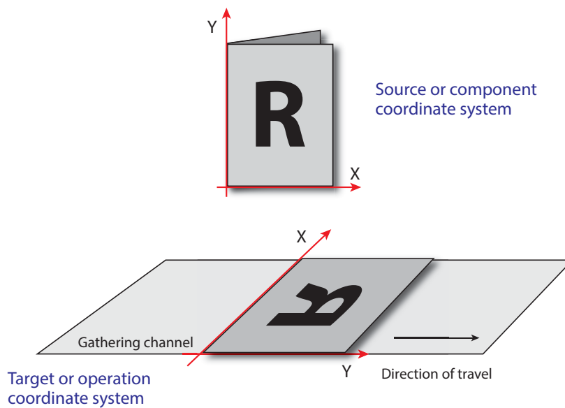
Figure 8-29: Coordinate system used for Gathering
