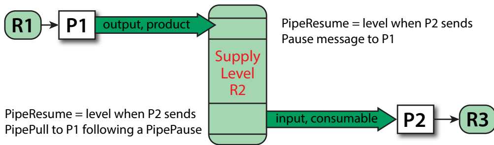
Figure 4-5: Example of a pipe resource linking two processes via push
