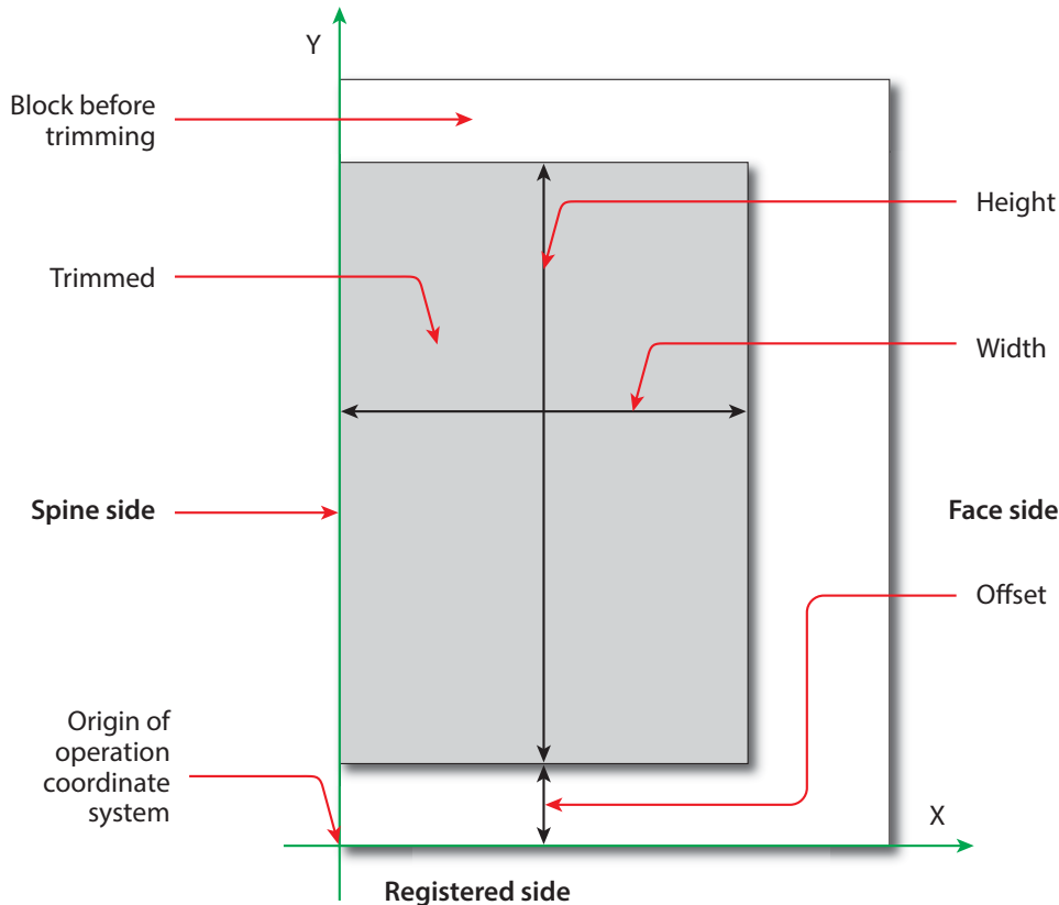
Figure 6-16: Parameters and coordinate system used for trimming
