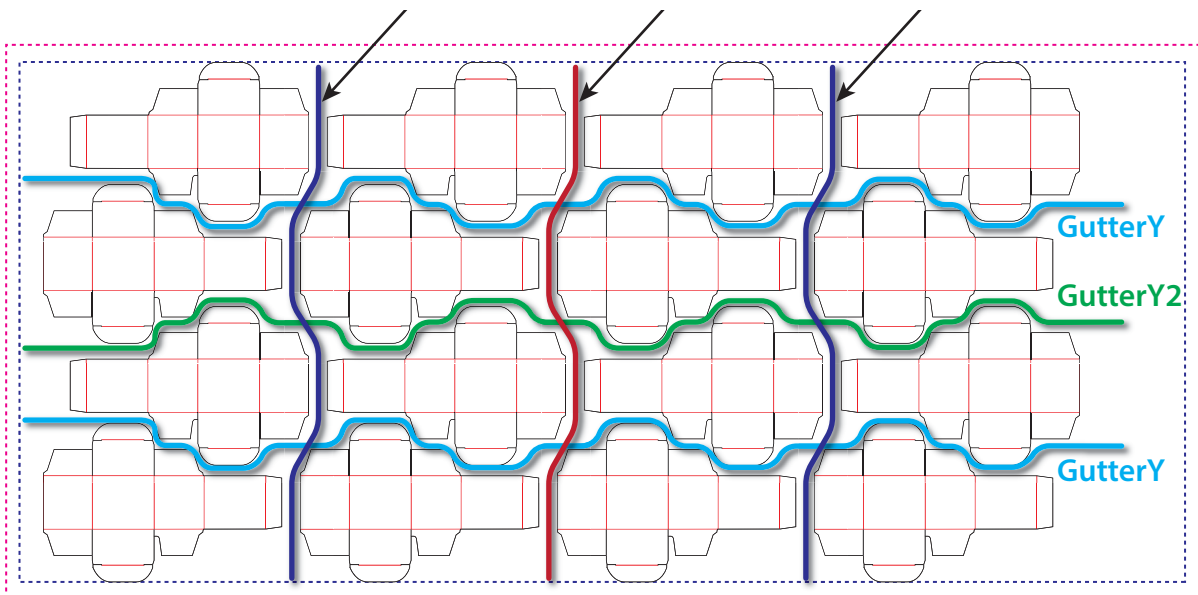
Figure 8-25: RepeatDesc/@GutterX2 and @GutterY2: Secondary Gutters
