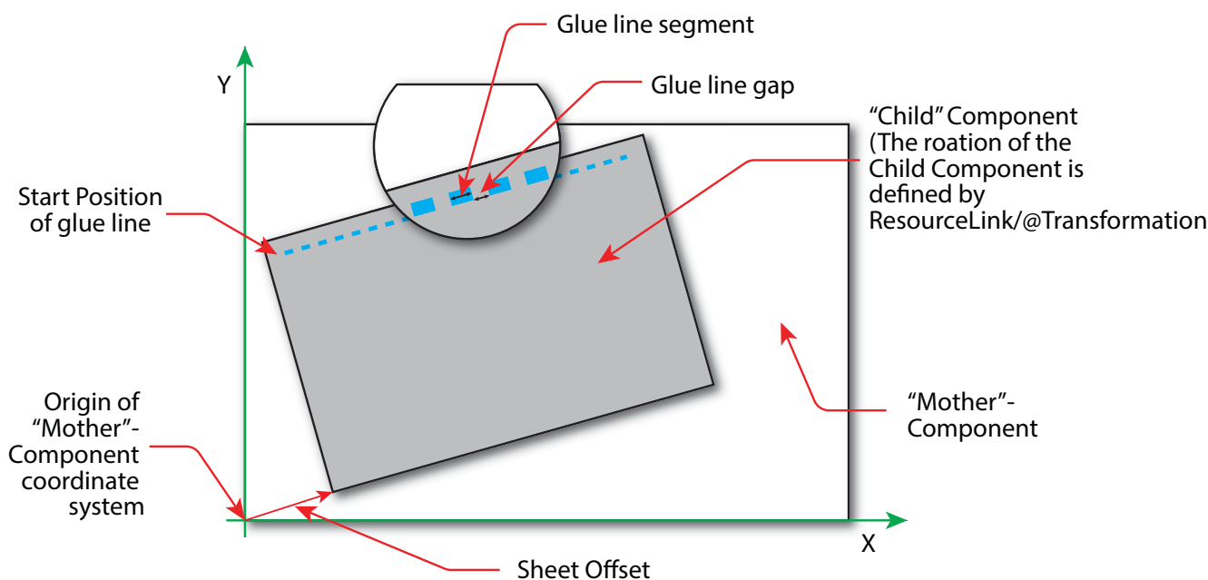
Figure 6-11: Parameters and coordinate system used for Inserting
