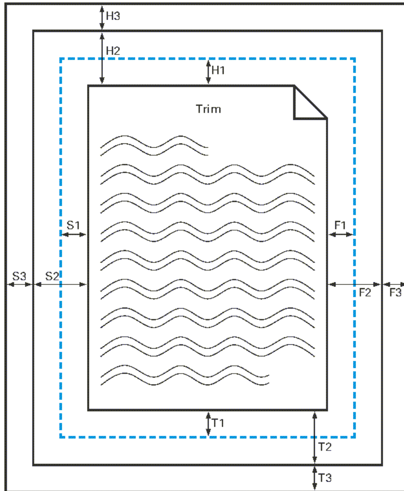
Figure 8-66: Definition of margins in StripCellParams
