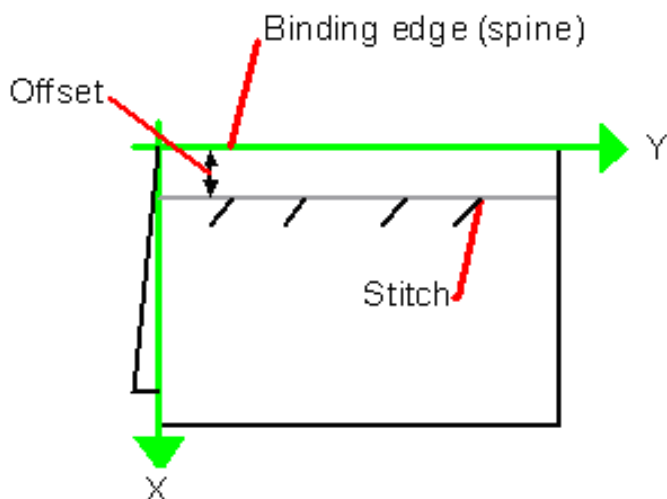
Figure 8-68: Parameters and coordinate system used for side sewing
