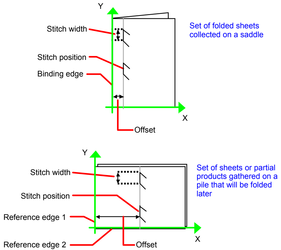
Figure 8-59: Parameters and coordinate system used for Stitching
