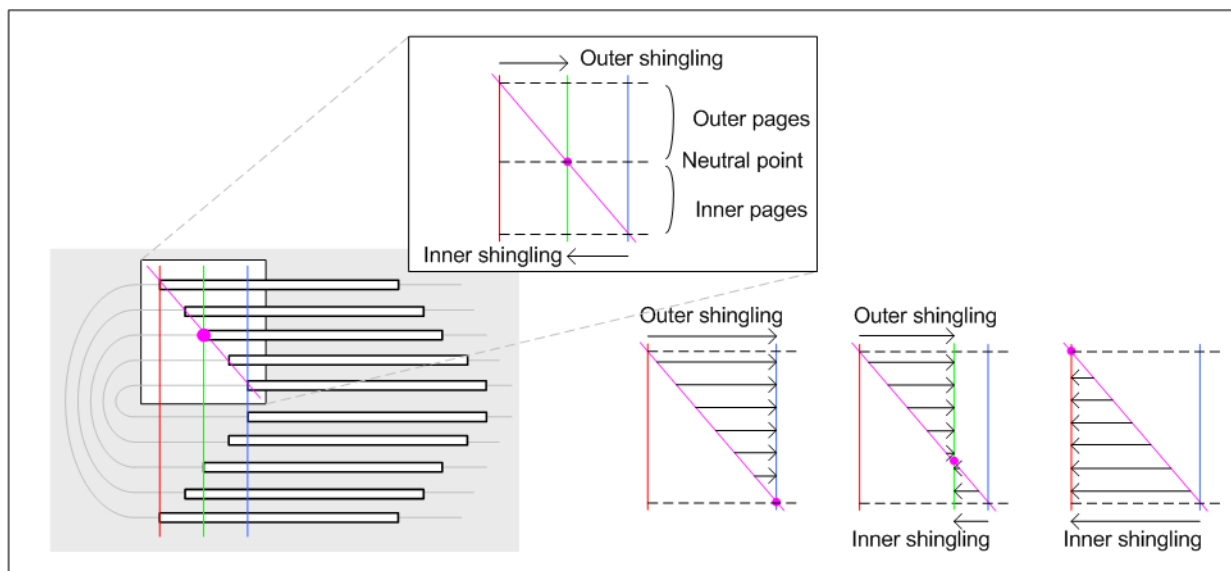
Figure 8-64: Shingling for Stripping – Details
