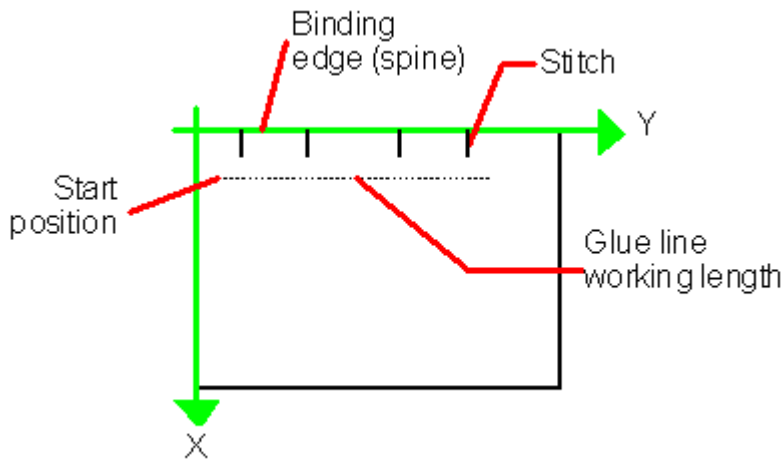
Figure 8-66: Parameters and coordinate system used for thread sewing
