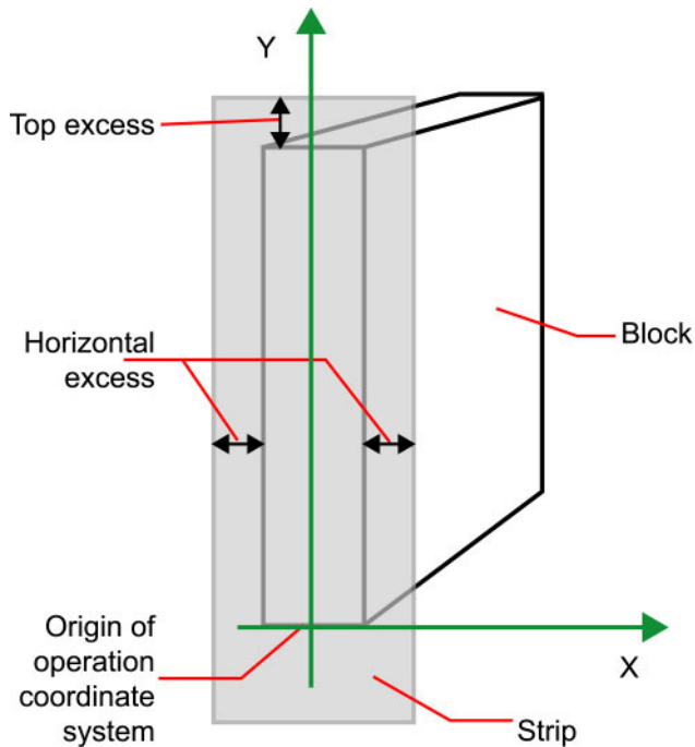
Figure 8-52: Parameters and coordinate system for the SpineTaping Process
