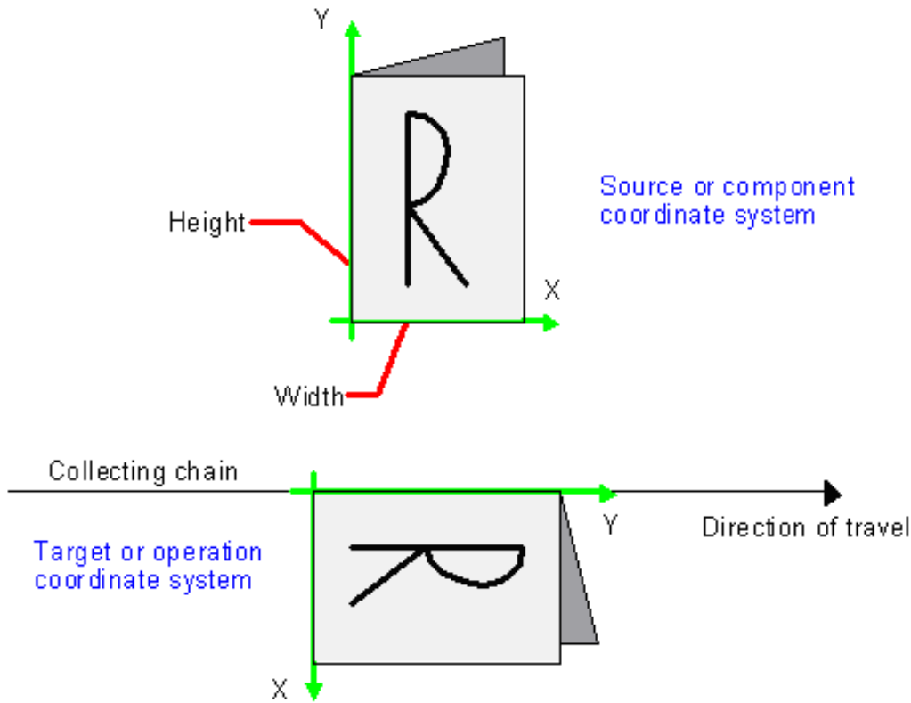
Figure 8-18: Coordinate systems used for collecting
