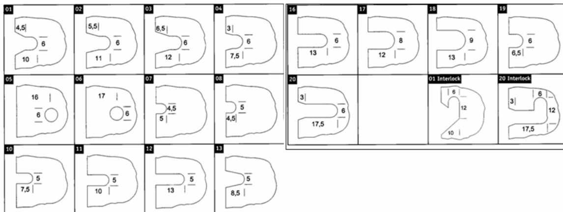
Figure 8-43: Types of Interlocks for Flexo Sleeve a
