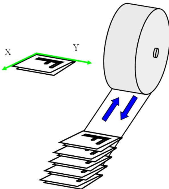
Figure 8-47: PrintRollingParams Coordinate System
