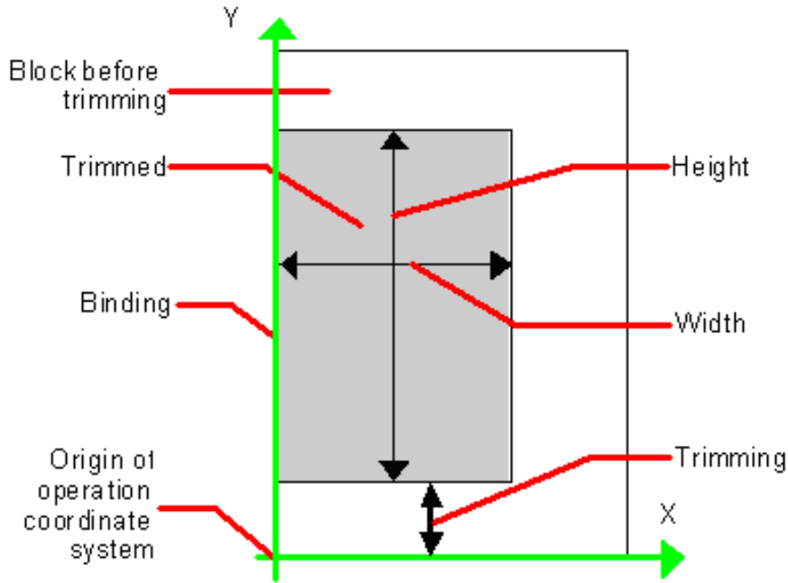
Figure 8-69: Parameters and coordinate system used for trimming
