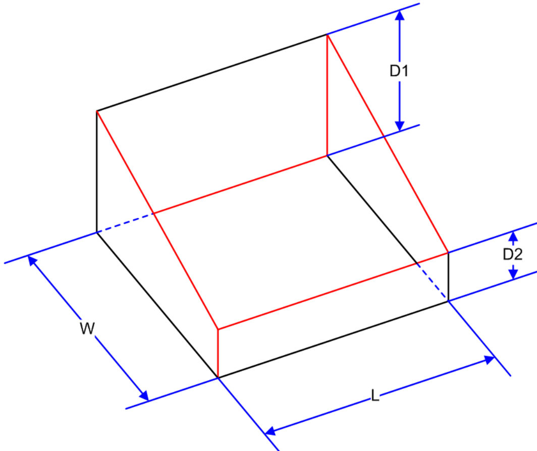
Figure 8-49: ShapeTemplate Example 2
