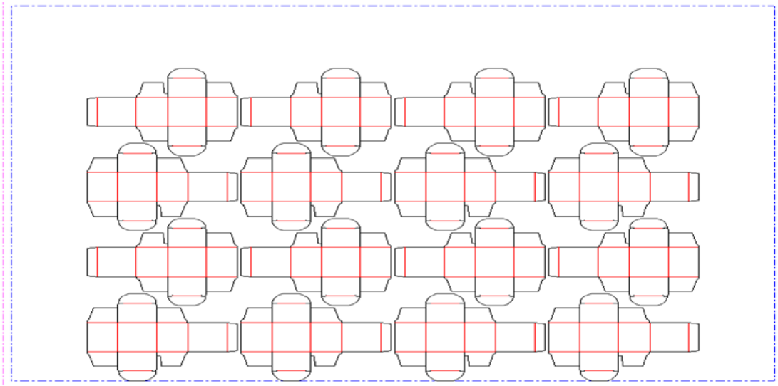
Figure 8-27: RepeatDesc/@LayoutStyle = "Reverse2ndRowAligned"
