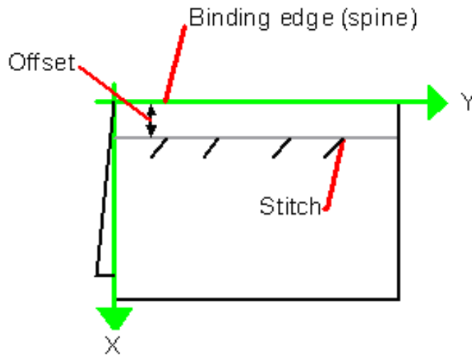
Figure 8-67: Parameters and coordinate system used for side sewing
