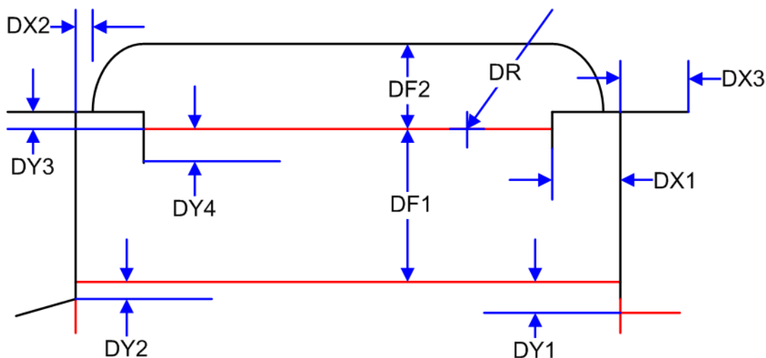
Figure 8-50: ShapeTemplate Example 3
