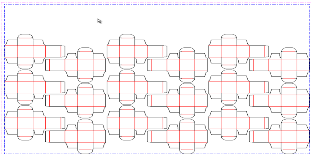
Figure 8-28: RepeatDesc/@LayoutStyle = "Reverse2ndColumn"
