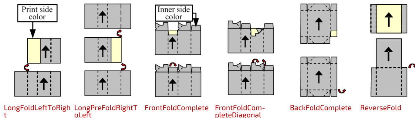
Figure 8-7: Folding examples for some values of BoxFoldAction/@Action
