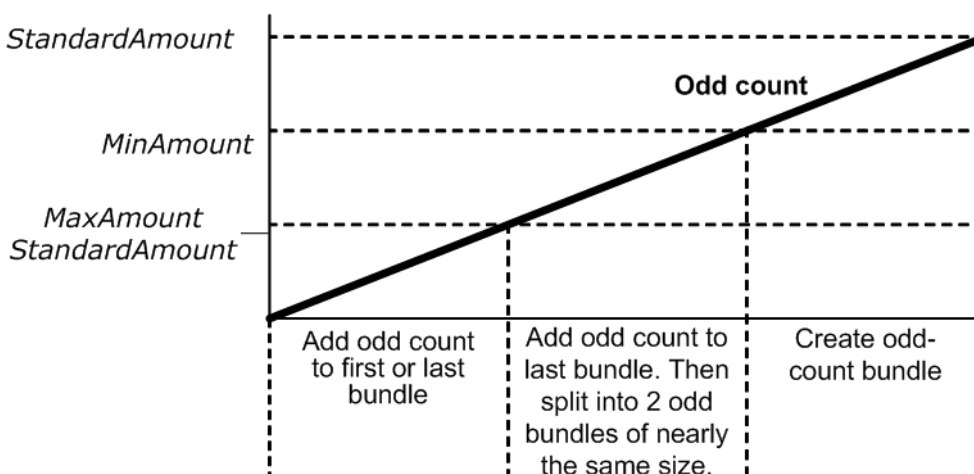
Figure 8-55: Odd count handling for a Bundle
