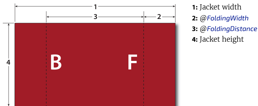
Figure 6-25: Parameters and coordinate system for jacketing
