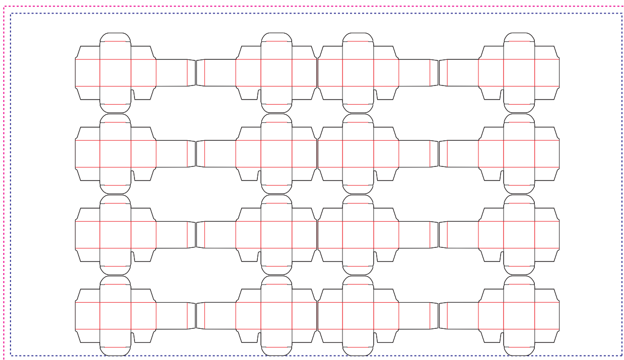
Figure 6-21: RepeatDesc/@LayoutStyle = "Reverse2ndColumnAligned"
