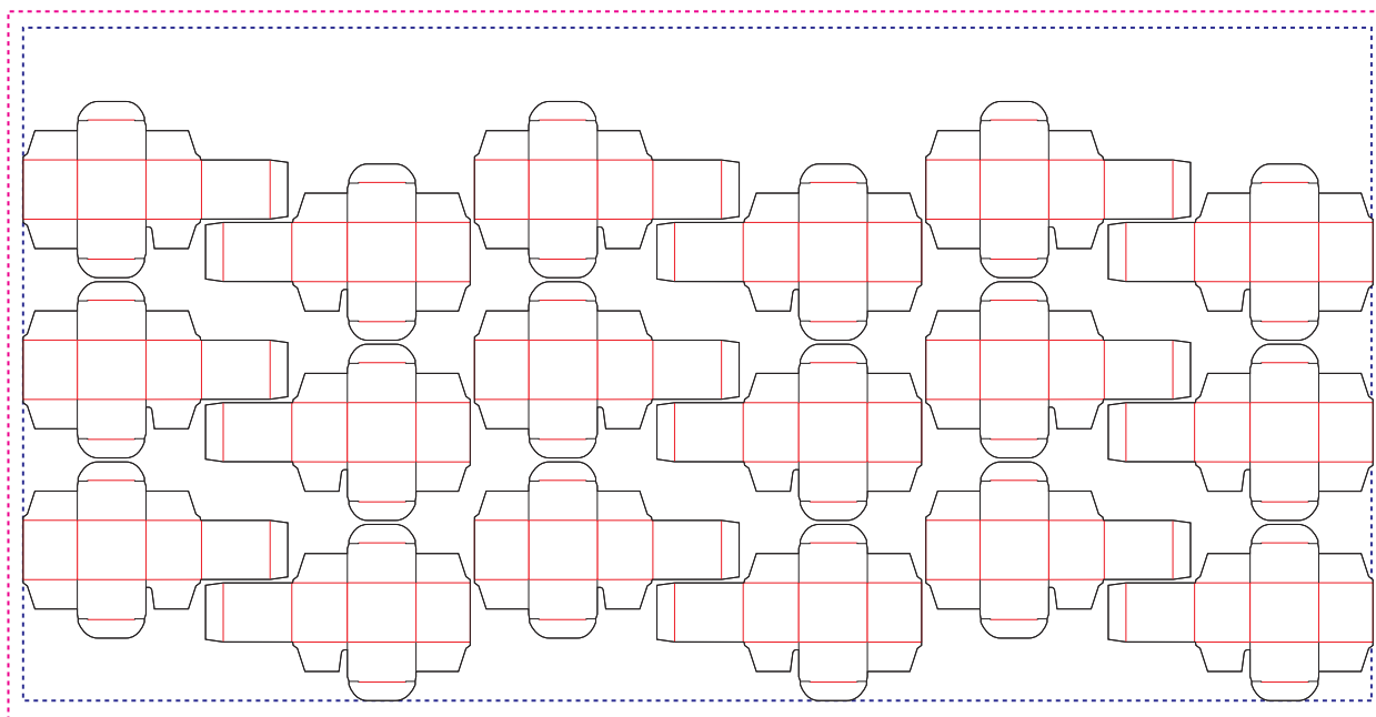
Figure 6-20: RepeatDesc/@LayoutStyle = "Reverse2ndColumn"
