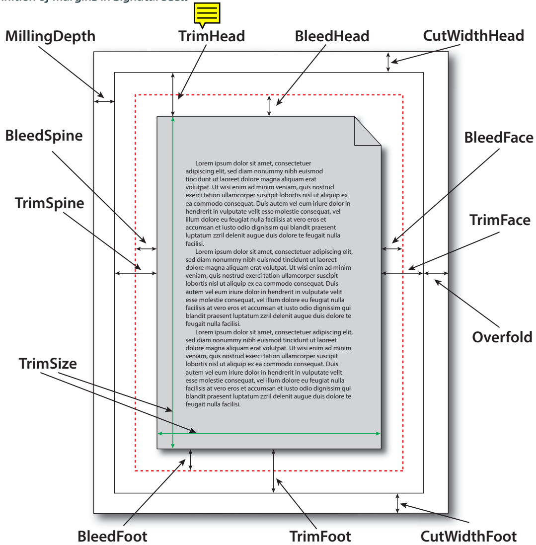
Figure 6-3: Definition of margins in SignatureCell
