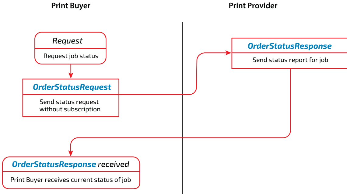
Figure 6-8: Job Tracking without Subscription
