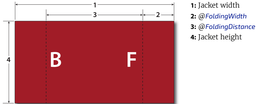
Figure 8-31: Parameters and coordinate system for jacketing
