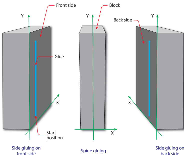
Figure 8-29: Parameters and coordinate system for GlueApplication
