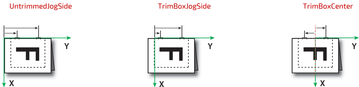
Figure 6-39: Stitching coordinate system for \bar{a} StitchOrigin values
