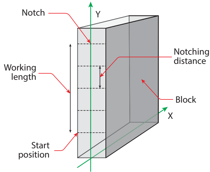
Figure 6-35: Parameters and coordinate systems for the SpinePreparation process
