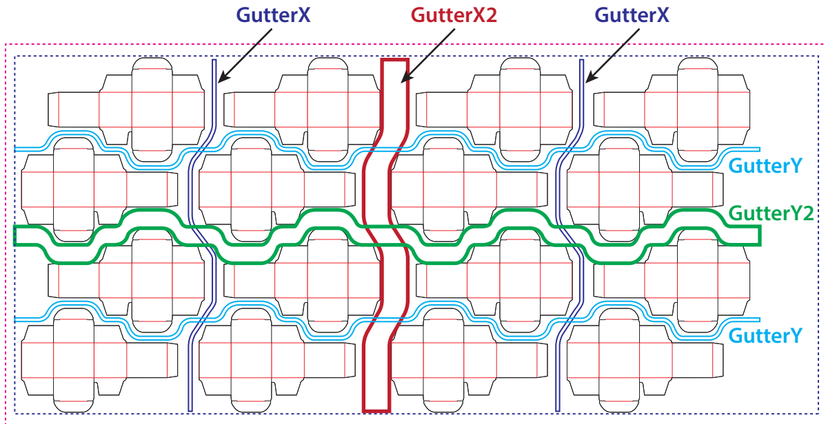
Figure 6-20: RepeatDesc using Secondary Gutters
