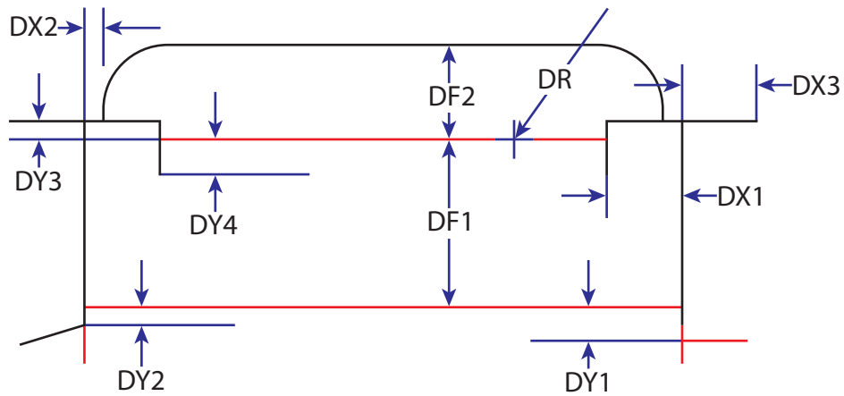
Figure 6-34: ShapeTemplate example 3
