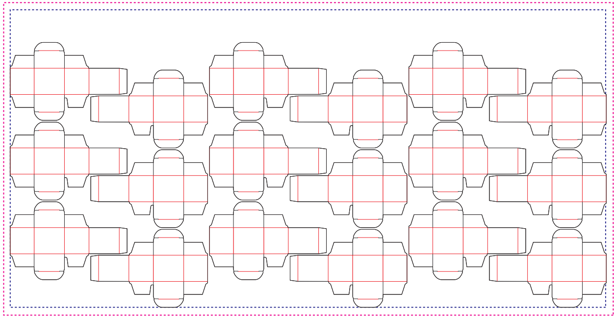
Figure 6-18: RepeatDesc/@LayoutStyle = "Reverse2ndColumn"
