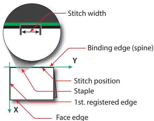
Figure 6-37: Parameters and coordinate system used for saddle stitching
