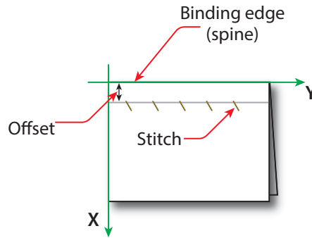
Figure 6-43: Parameters and coordinate system used for side sewing
