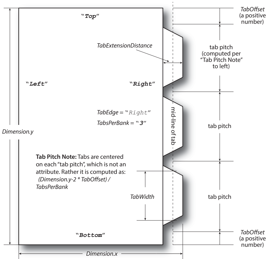
Figure 6-30: Diagram of a single bank of tabs
