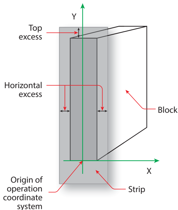
Figure 6-36: Parameters and coordinate system for the SpineTaping process
