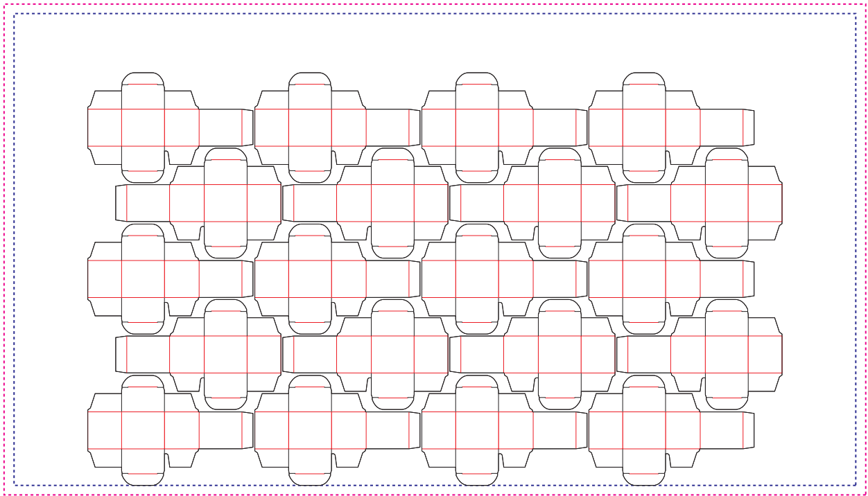
Figure 6-16: RepeatDesc/@LayoutStyle = "Reverse2ndRow"
