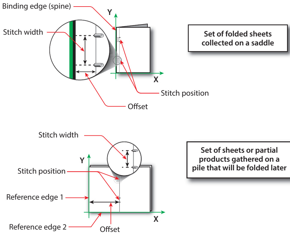
Figure 6-38: Parameters and coordinate system used for stitching
