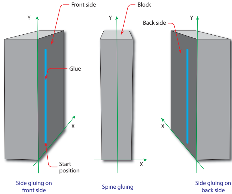
Figure 6-12: Parameters and coordinate system for glue application
