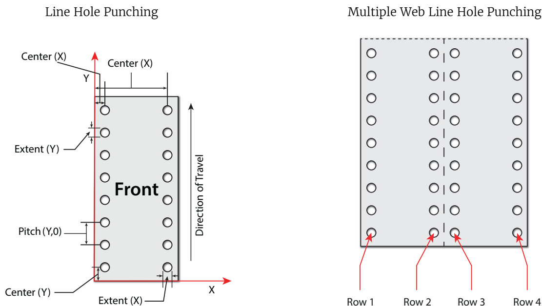
Figure 5-8: HolePattern parameters
