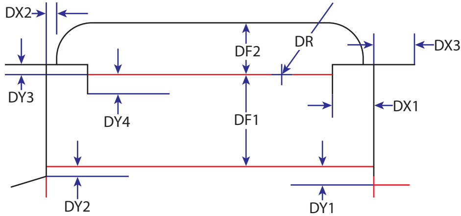
Figure 6-34: ShapeTemplate example 3
