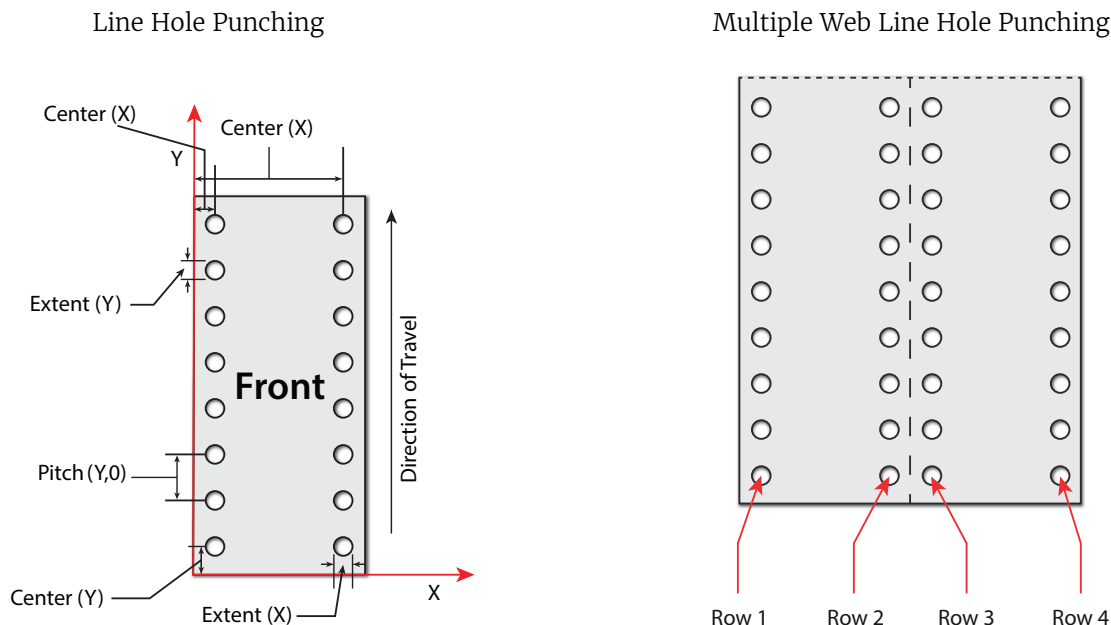
Figure 5-8: HolePattern parameters
