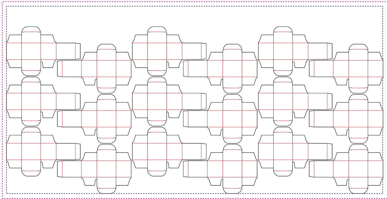
Figure 6-18: RepeatDesc/@LayoutStyle = "Reverse2ndColumn"
