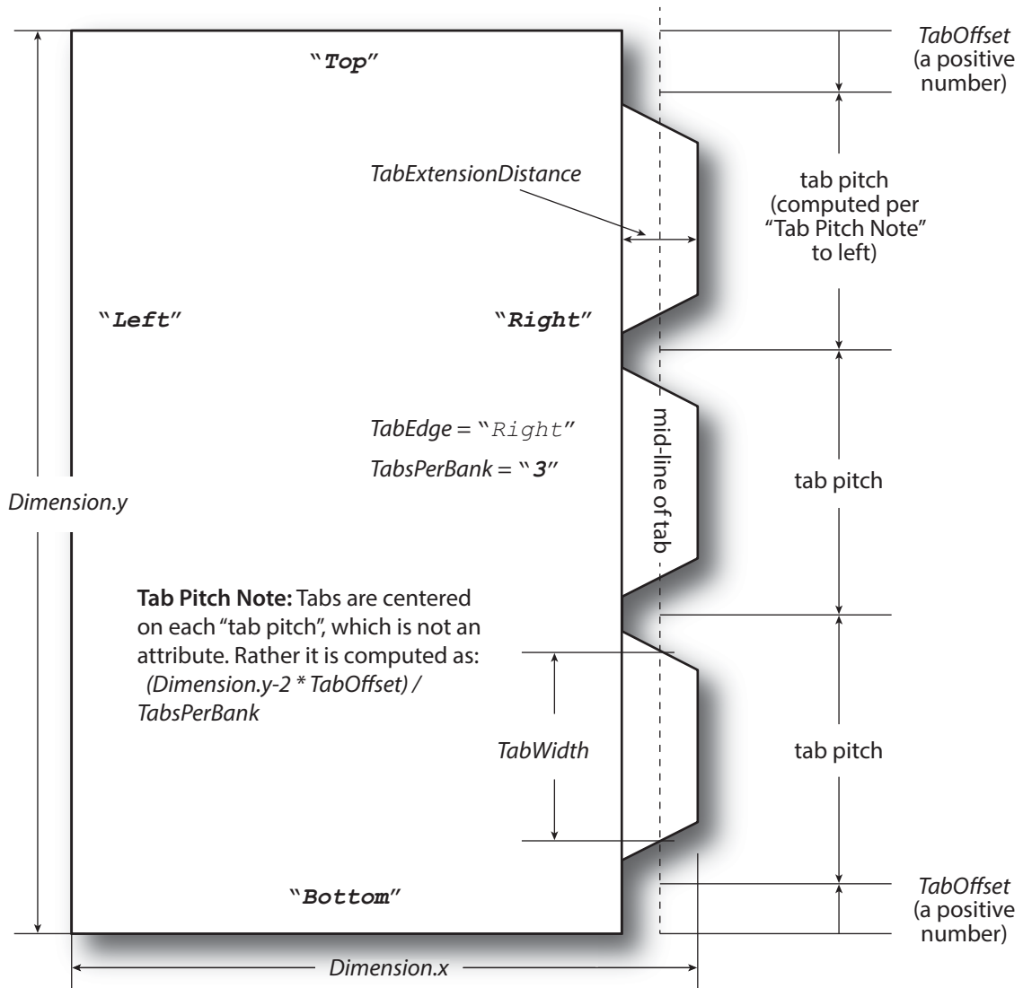
Figure 6-31: Diagram of a single bank of tabs
