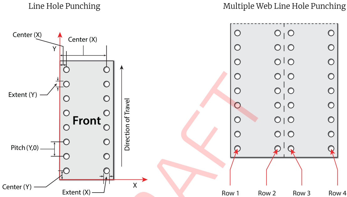
Figure 6-9: Hole parameters
