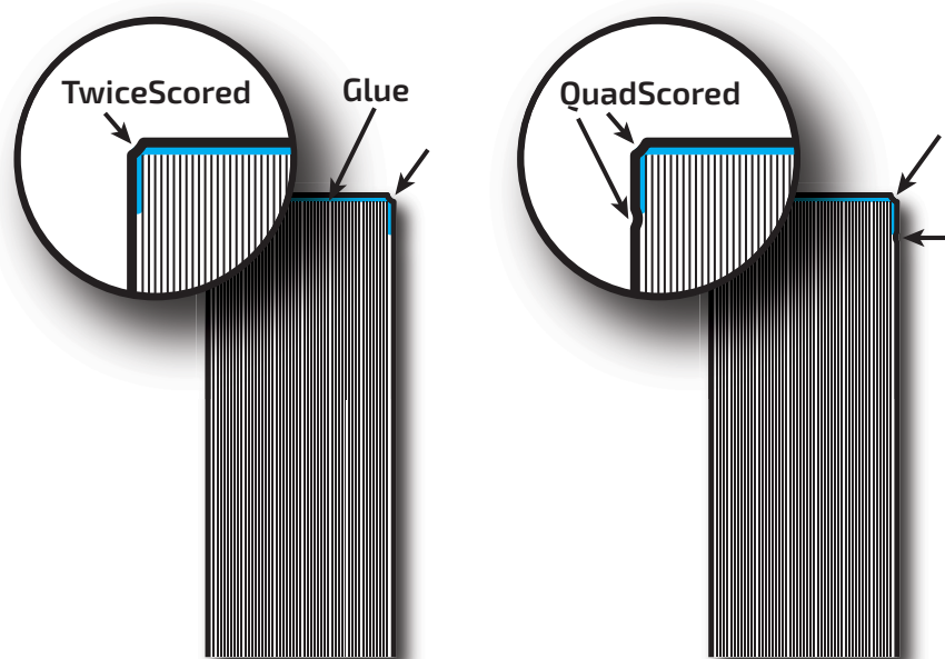
Figure 7-4: Scoring for soft cover binding
