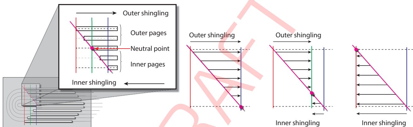
Figure 6-28: Shingling for stripping – details
