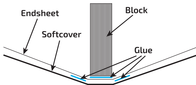
Figure 4-4: Structure of a book with GlueProcedure = "SideOnly" (Layflat)
