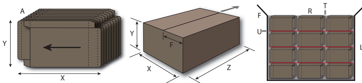
Figure 6-6: Box packing
