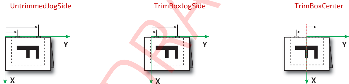
Figure 6-42: Stitching coordinate system for @StitchOrigin values
