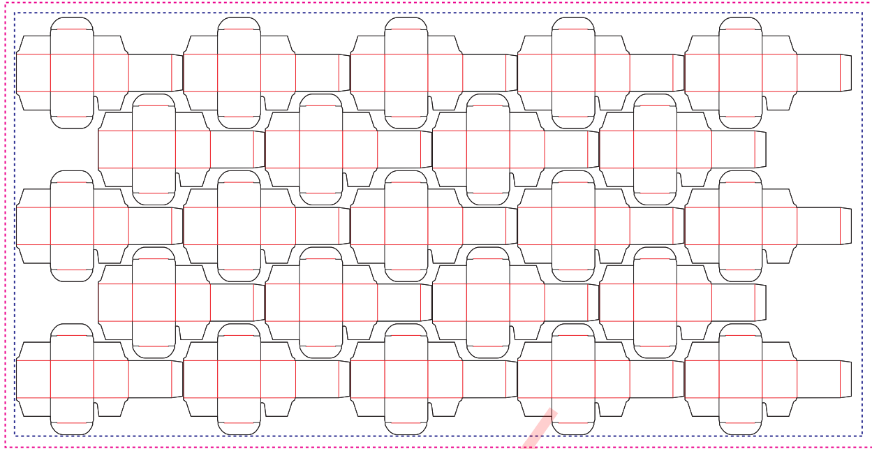
Figure 6-17: RepeatDesc/@LayoutStyle = "StraightNest"
