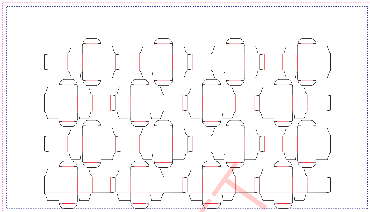
Figure 6-19: RepeatDesc/@LayoutStyle = "Reverse2ndRowAligned"
