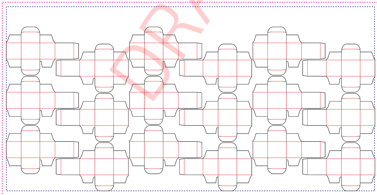
Figure 6-20: RepeatDesc/@LayoutStyle = "Reverse2ndColumn"
