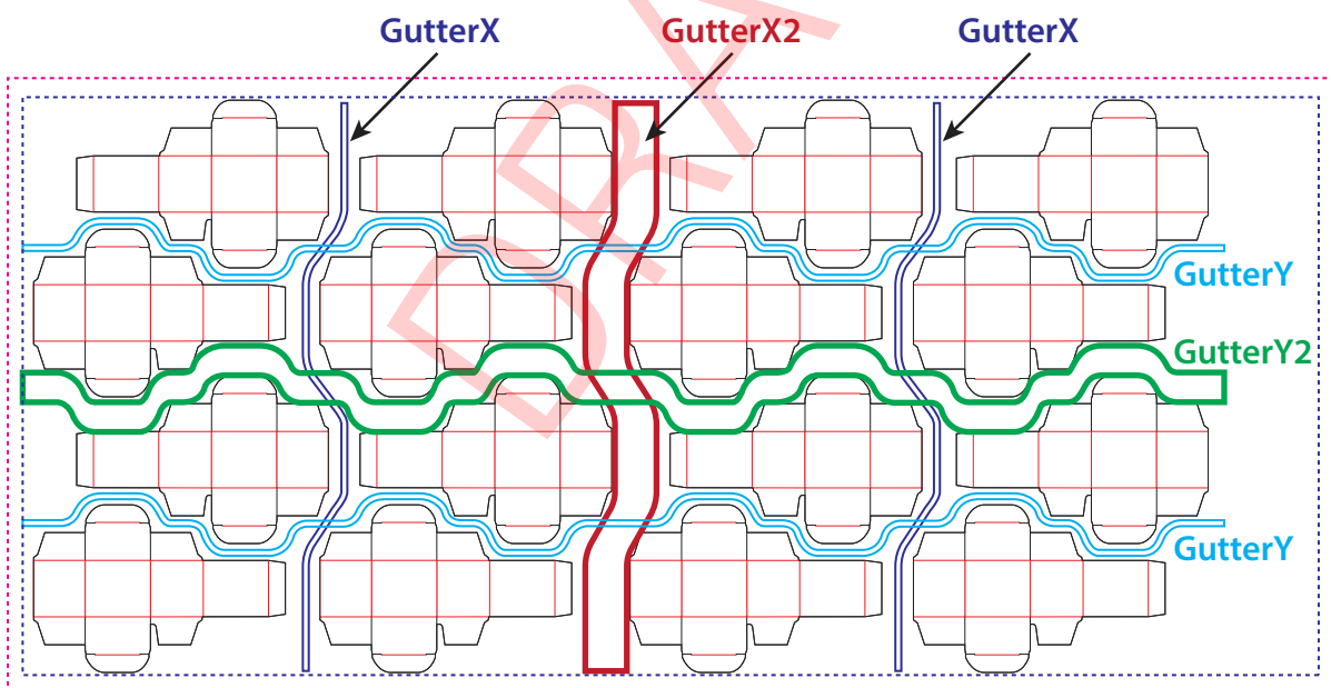
Figure 6-22: RepeatDesc using Secondary Gutters
